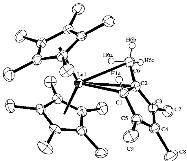
Figure 2. Thermal ellipsoid plot of [(\eta^5-C_5Me_5)_2Lu(\eta^3-C_5Me_4H)] ( 2 ) drawn at the 50% probability level. There are two independent molecules of 2 in the unit cell. The second independent molecule of 2 and hydrogen atoms except for H1a, H6a, H6b, and H6c are omitted for clarity.
